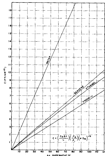
Fig. 7. Bubble growth-rate constants for superheated systems at 1 atm.
