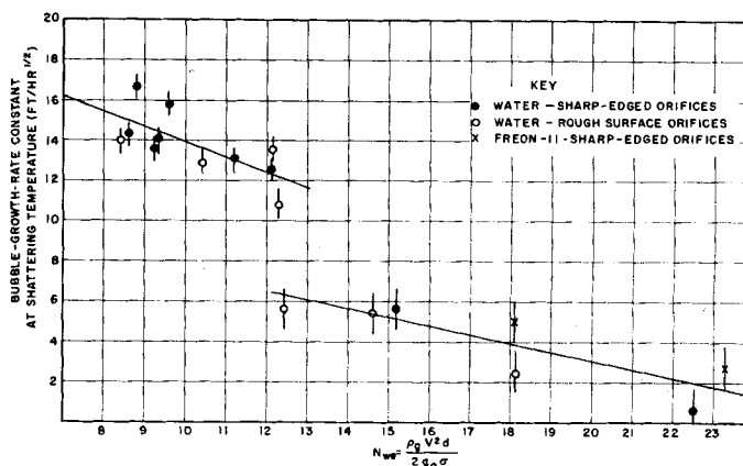
Fig. 8. Effect of Weber number on water and Freon-11 jet breakup.
